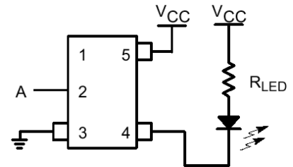
Figure 8. LED Driver
