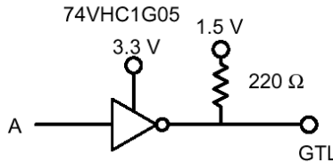
Figure 9. GTL Driver
